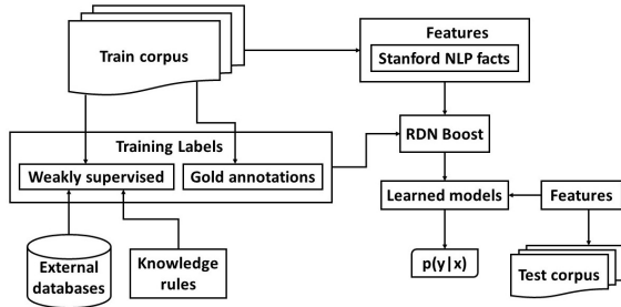
Figure 1: Full RDN relation extraction pipeline
