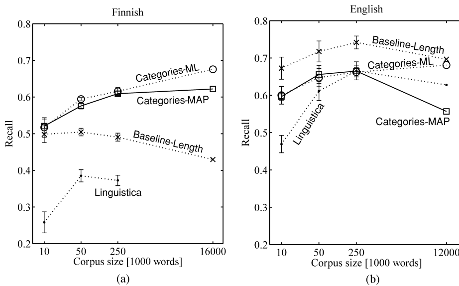
Fig. 8. Recall of discovered morpheme boundaries obtained by the algorithms on (a) Finnish and (b) English data. Standard deviations are shown as intervals around the data points. Precision (Figure 7) measures the accuracy of the proposed splitting points, while, recall describes the coverage of the splits.
