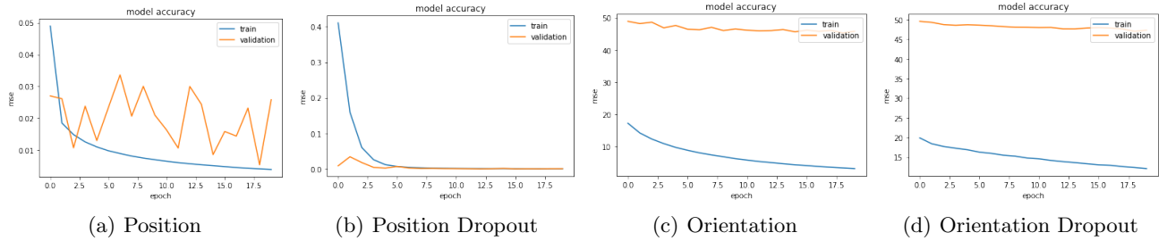
Figure 4. Training and validation results with s-fold cross validation, and when s=10 . The graphs (a) & (b) show the translation loss smooths out when using dropout in training. A similar effect can be seen with the orientation in (c) & (d). Note that dropout is always turned off during validation and testing.
