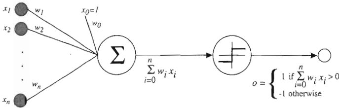
FIGURE 4.2 A perceptron.
