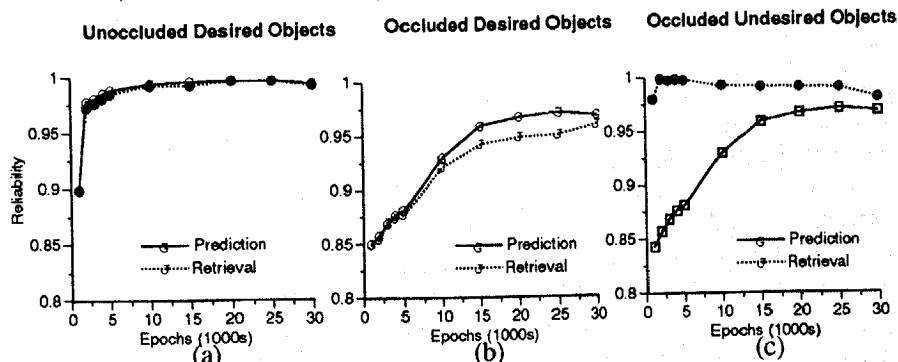
Figure 3: Network performance on predictive visual pursuit and manual retrieval to (a) an unoccluded desired object, (b) an occluded desired object, and (c) an occluded undesired object.
