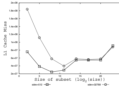
(a) L1 cache misses versus size of the subset.
