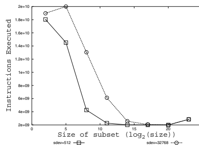
(c) Number of instructions executed versus size of the subset.
