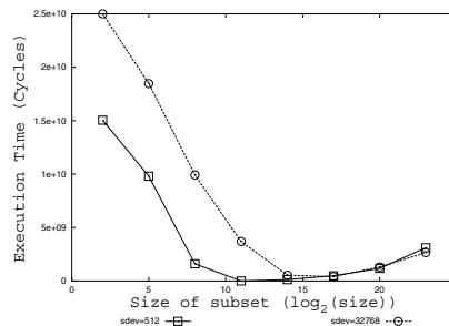
(d) Cycles executed versus size of the subset.
