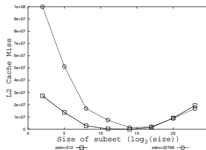
(b) L2 cache misses versus size of the subset.
