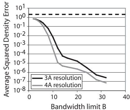
Figure 5: The average squared density difference between a region of sampled density and the bandwidth-limited region. The dotted line shows the error between two randomly selected regions.
