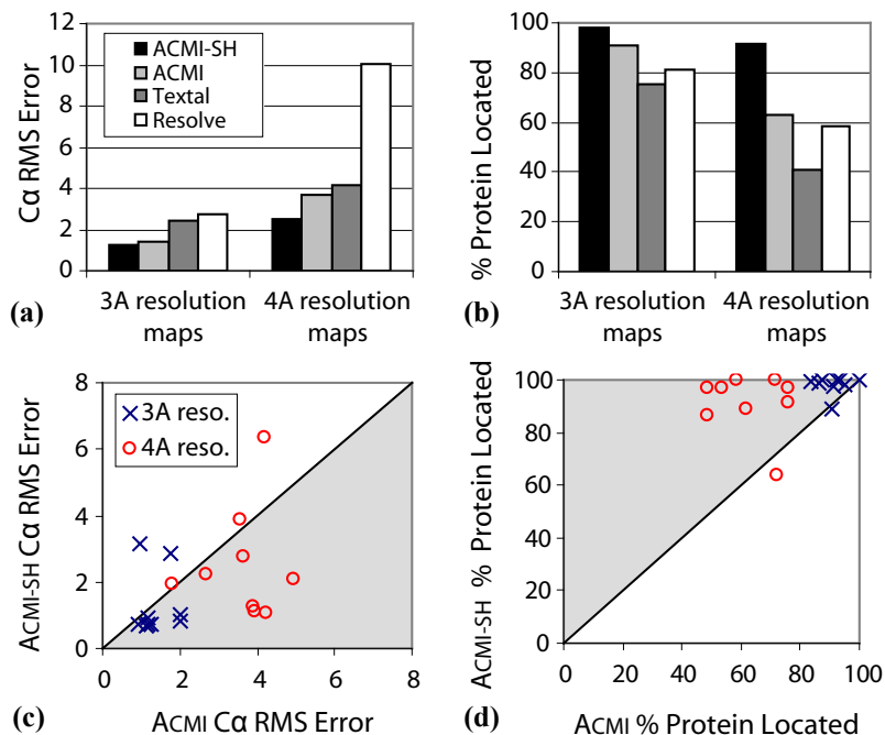
Figure 9: Comparing ACMI-SH’s protein models with three other methods. (a) The average C \alpha RMS error and (b) percentage of amino acids located. Scatter plots compare ACMI’s performance with ACMI-SH’s on (c) RMS error and (d) percentage of amino acids located. For (c) and (d), the shaded region indicates superior performance by ACMI-SH.
