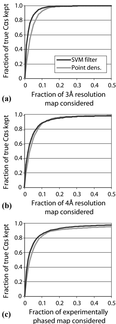
Figure 7: A comparison of two different filters: the best simple filter from Figure 6, the point-density filter, and a filter based on a support vector machine (SVM). Filter performance is compared on (a) 3Å, (b) 4Å resolution and (c) varied resolution, experimentally phased density maps.
