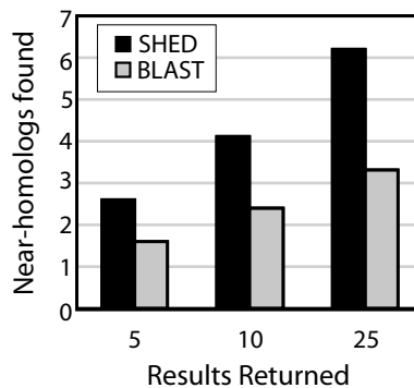
Figure 10: The average number of structural homologs found by SHED and BLAST when considering the top 5, 10, and 25 results returned. A near-homolog is a returned result that is also returned in the top 5, 10, or 25 results of DaliLite.
