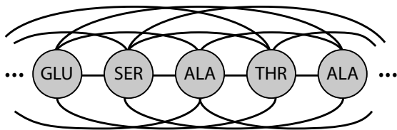
Figure 2: The undirected graph corresponding to the protein’s Markov-field model. The probability of some backbone model is proportional to the product of potential functions: one associated with each vertex, and one with each edge in the fully connected graph.
