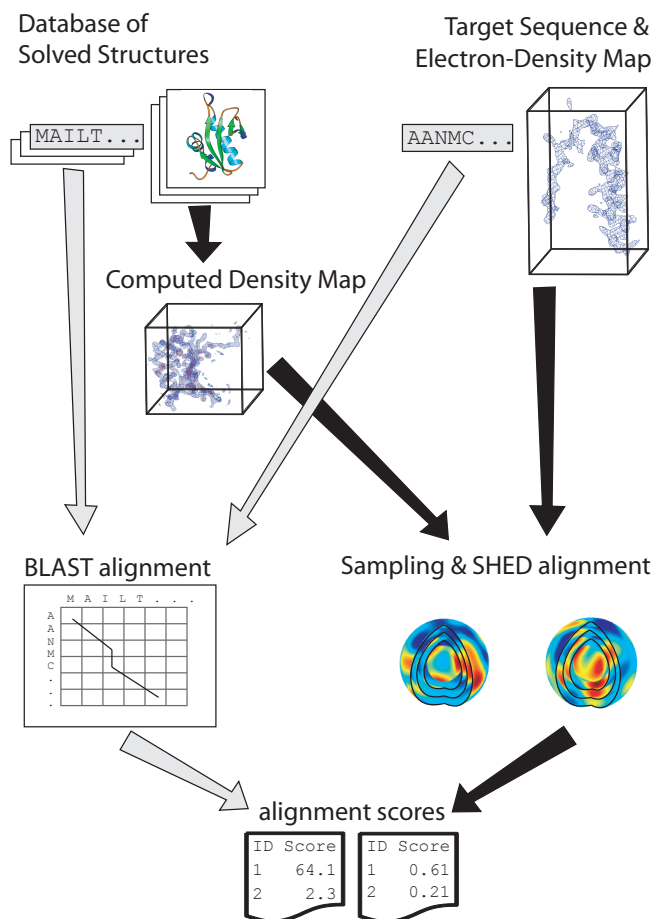
Figure 4: A comparison of two homology-search algorithms. SHED (lower right) compares a target protein’s electron-density map against a database of solved protein structures. This algorithm is similar to that in Figure 3, except we compare the whole protein structure against the density map instead of just small fragments. BLAST (lower left) considers the sequences of the solved structures and target protein, using a dynamic programming model to measure similarity between two sequences. Black arrows show the movement of density information, while grey arrows indicate the use of sequence information.
