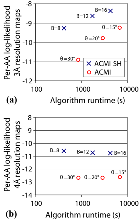
Figure 8: A comparison of ACMI-SH’s and ACMI’s template matching on (a) 3Å and (b) 4Å resolution maps, in terms of average per-amino-acid log-likelihood of the true trace (higher values are better).
