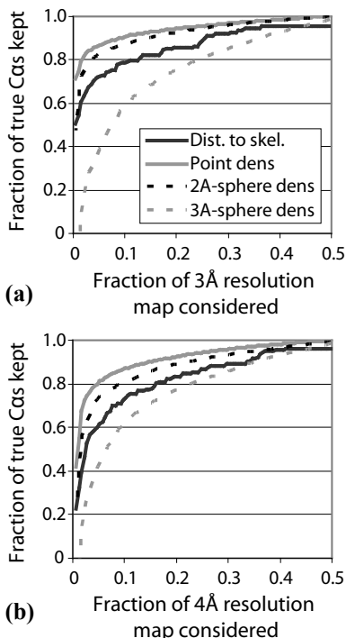
Figure 6: A comparison of four different filters for quickly eliminating some portion of points in the density map. Filter performance is compared on (a) 3Å and (b) 4Å resolution density maps.
