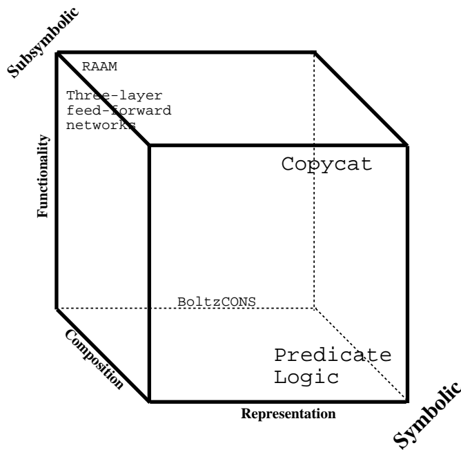
Figure 1: Subsymbolic/symbolic continuum : This figure illustrates the three dimensional space of paradigms defined by the three characteristics from Table 1: representation (across the bottom), composition (extending out), and functionality (up the side). The Gap between the symbolic (front, lower, right corner) and subsymbolic (back, upper, left corner) paradigms can be viewed as the central region of the cube. Five models are shown in their approximate position in the space. Font size reflects distance from the front of the box.
